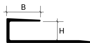
Aluminum - LTR60 B = 11 mm
