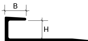
Aluminum - LTR50 B = 6 mm
